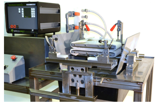
Semi-automated Workstation
